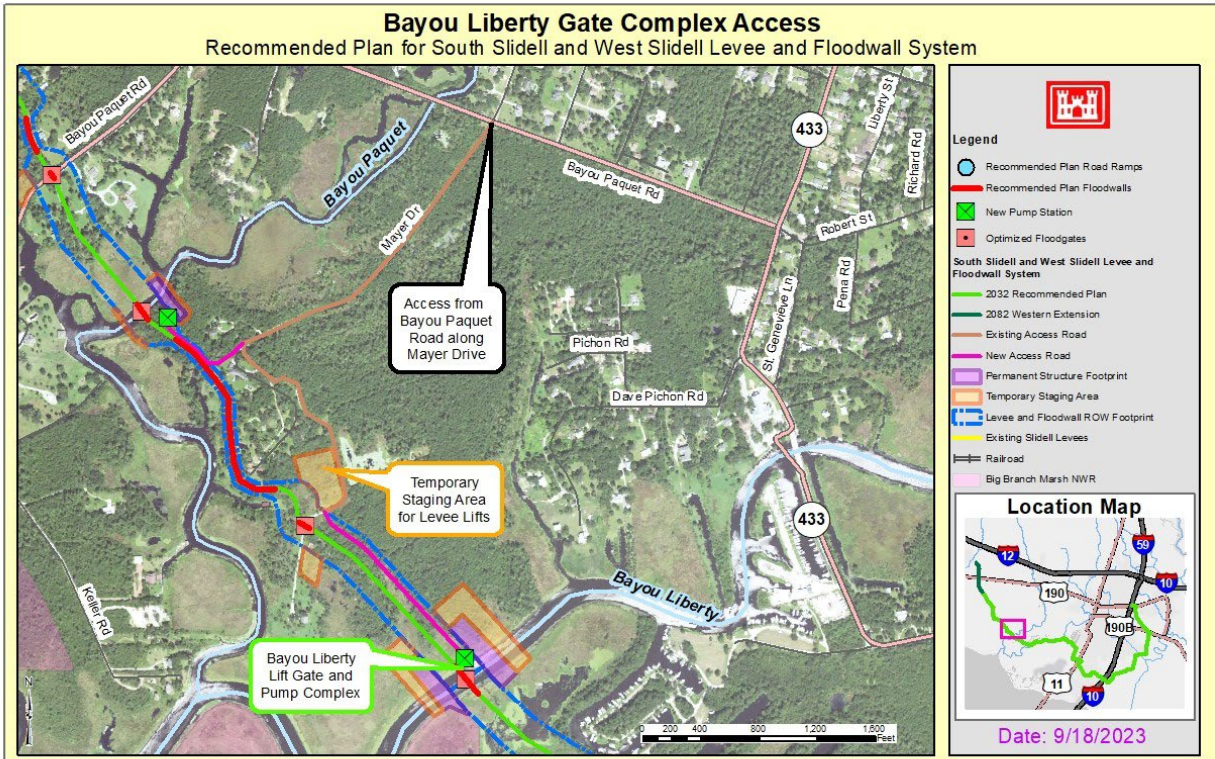
Figure D6:1-9. ROW, Access, and Staging Areas for the Bayou Liberty Pump Station and Floodgate
