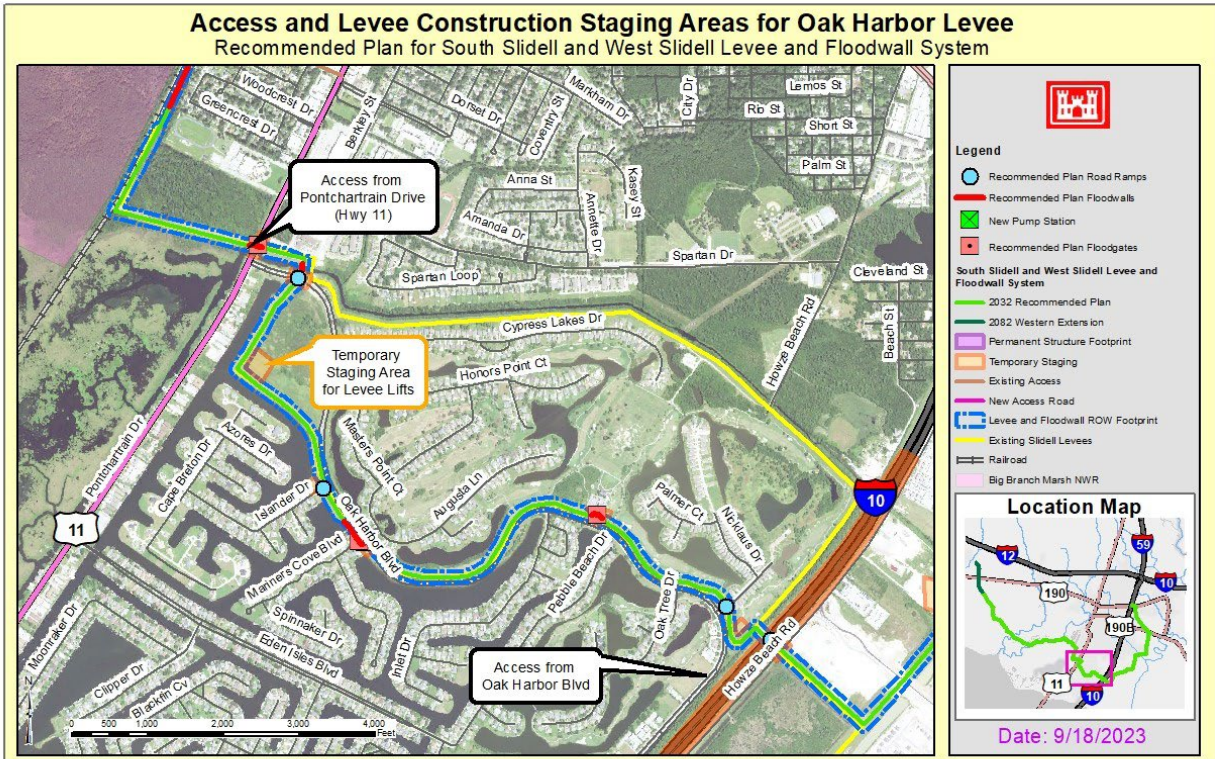
Figure D6:1-13. ROW, Access, and Staging Areas for Oak Harbor Levee
