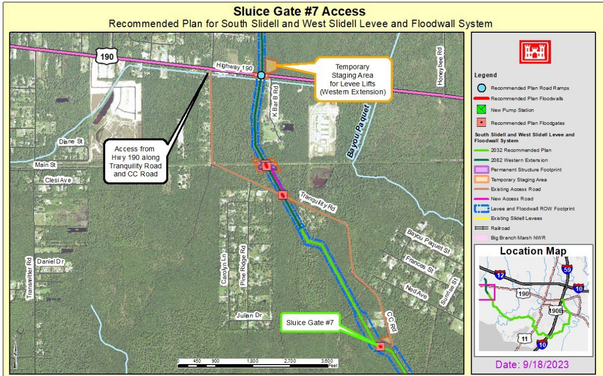
Figure D6:1-4. ROW, Access, and Staging Areas for Sluice Gate # 7
