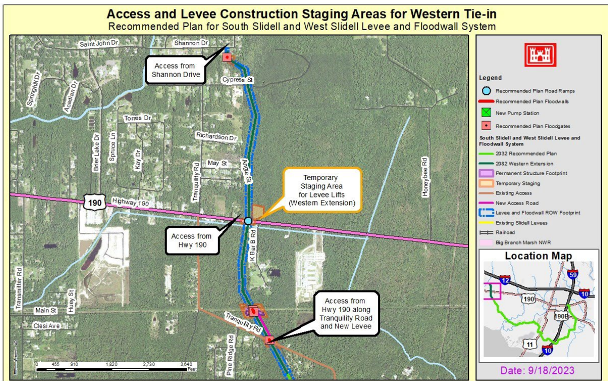
Figure D6:1-1. ROW, Access, and Staging Areas for Western Tie-In
